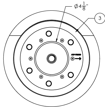
DETAIL A SCALE 1 : 3 GASKET REMOVED FOR CLARITY
